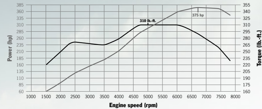
Boxster Spyder: 375 hp at 6,700 rpm, 310 lb.-ft. between 4,750 and 6,000 rpm
